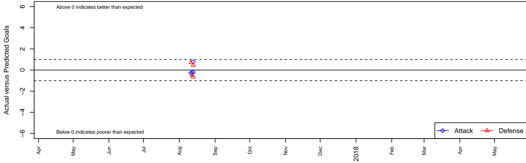
Bend FC Timbers Green B99 Dots are actual minus expected GF (blue circles) and GA (red triangles). Blue line is smoothed change in attack strength. Red is smoothed change in defense strength.
